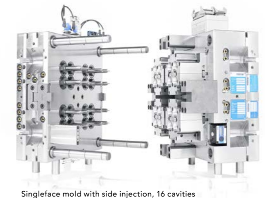
Singleface mold with side injection, 16 cavities
