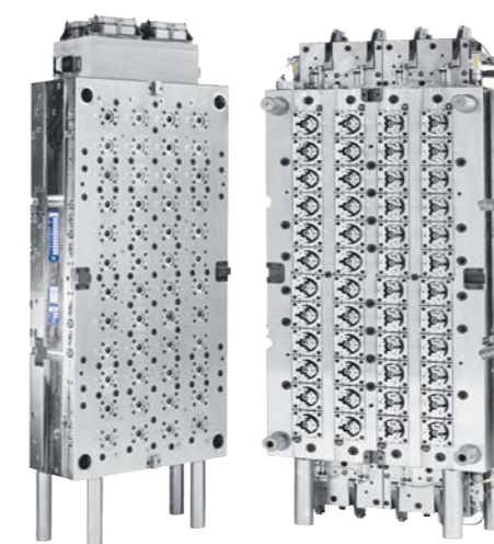
Singleface mold, 48 cavities
