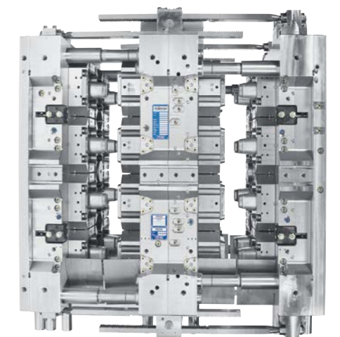
Stack mold, 2 x 8 cavities
