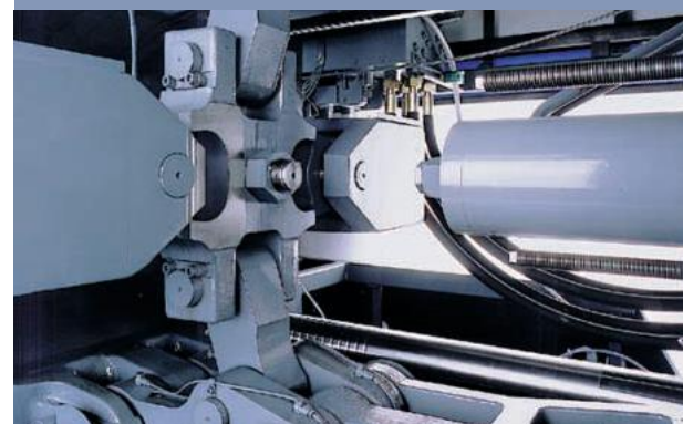
Fast and precise movements thanks to the 5-point toggle lever of solid design
