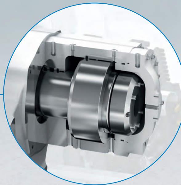
Pressure pads
